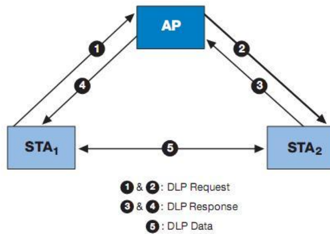
Figura A.7: Direct Link Protocol
