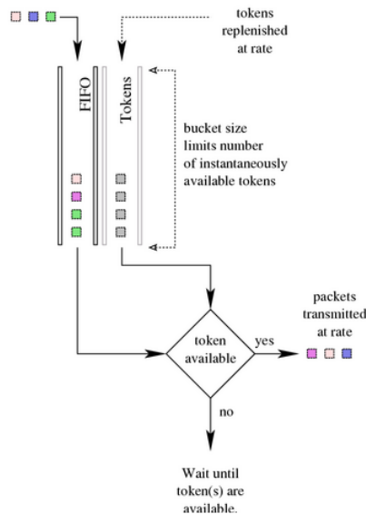
Figura E.2: Token Bucket Filter
