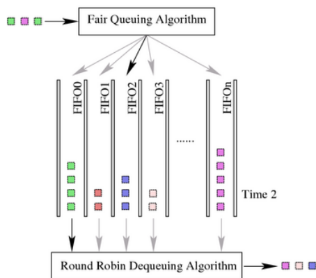
Figura E.3: Stochastic Fairness Queueing
